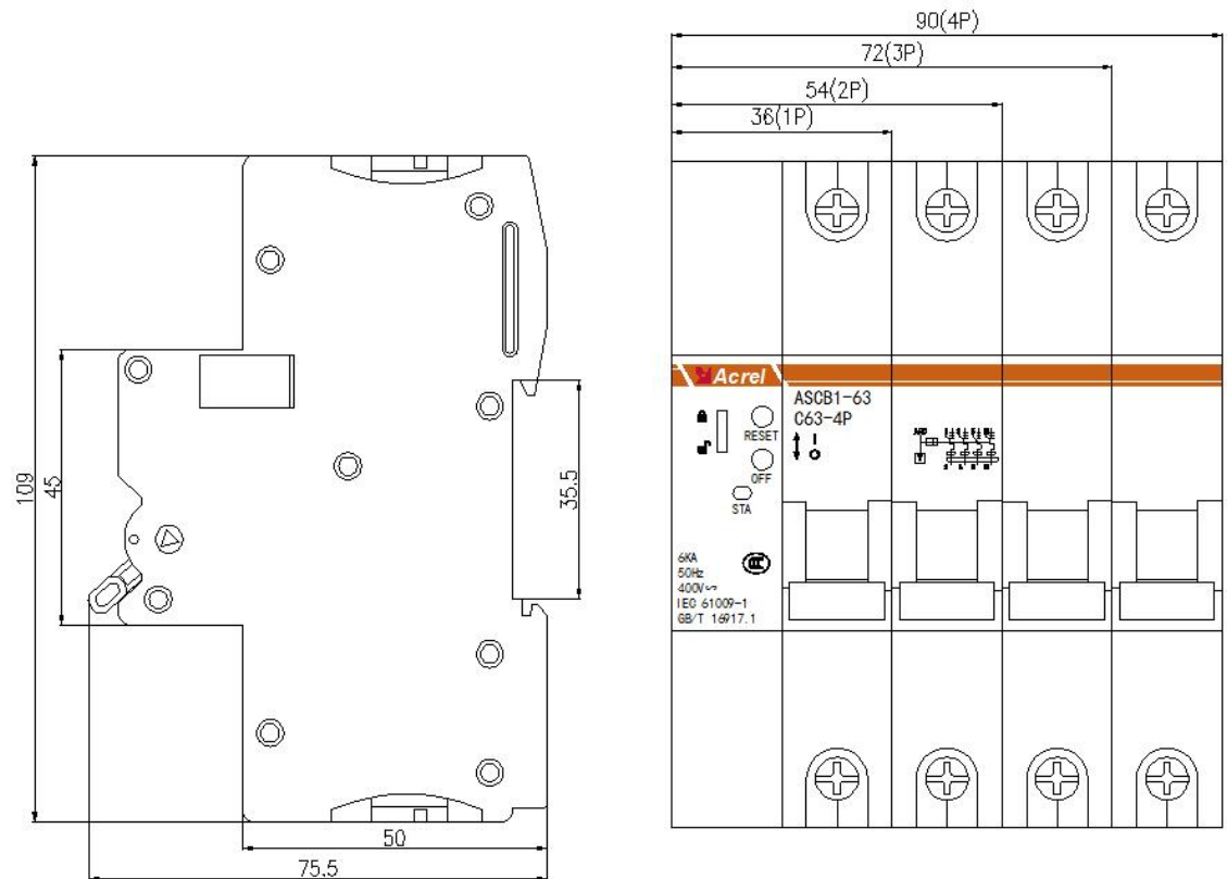
Figure 1 Outline dimensions of the intelligent micro circuit breaker
