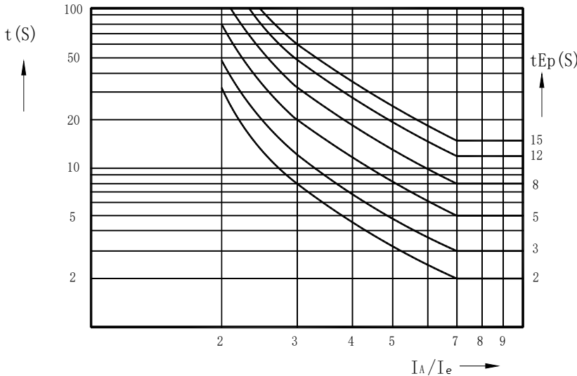
Fig.11 tE Protection delay to blocking current ratio I_A/I_e Current-time characteristic curve
