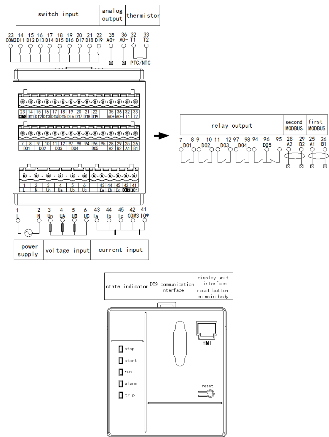
Fig. 9 ARD2F terminal arrangement
