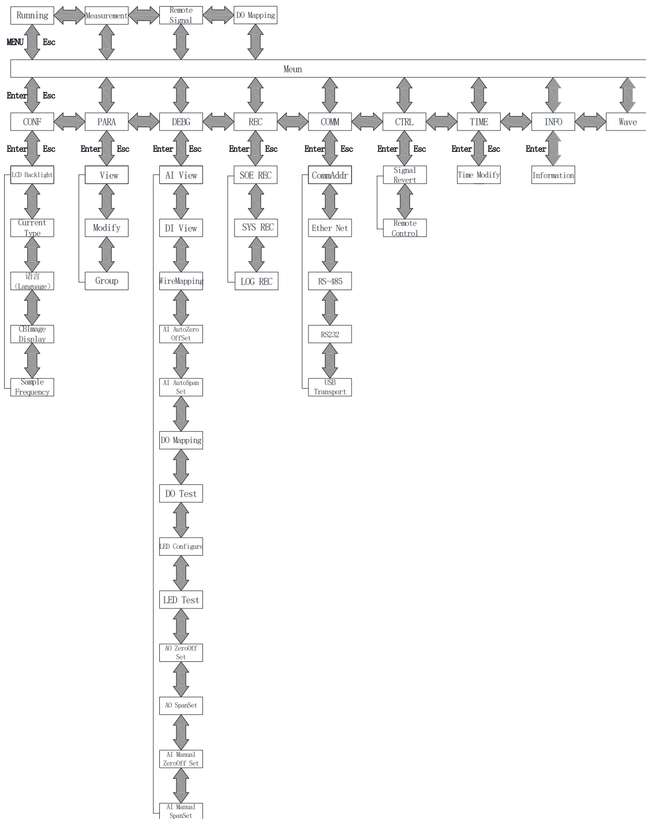
Figure 3.7 Navigation diagram
